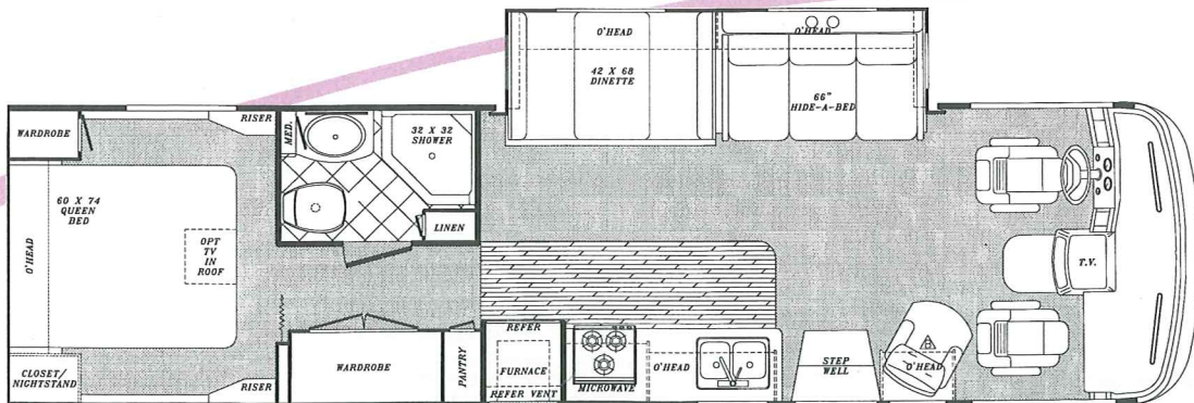
Model 8325 (Approx. 32'-7", 100" wide)
