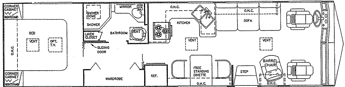
MODEL 8349 DIESEL
