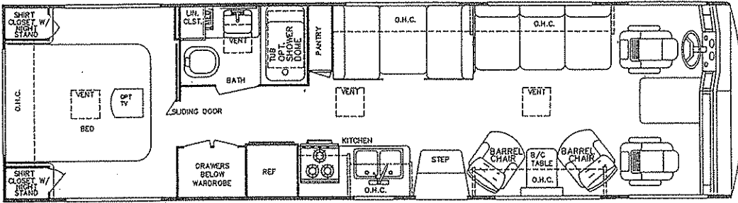
MODEL: 8344 GAS
