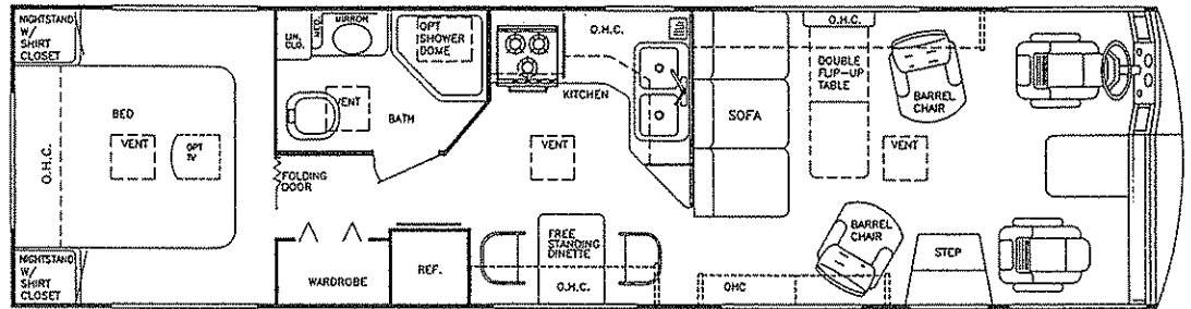
MODEL 8340 GAS
