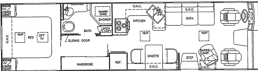
MODEL 8349 GAS
