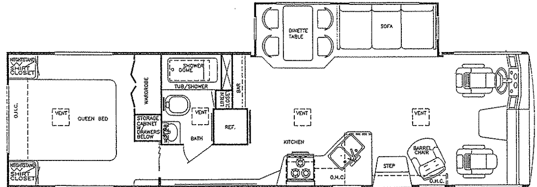
MODEL 8341 GAS
