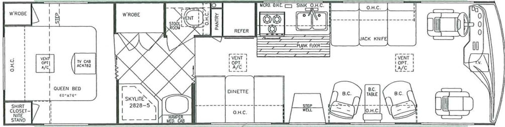
Model 8334 (Approx. 34' - 6", 101" wide)
