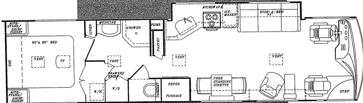
Model 8362 DIESEL
