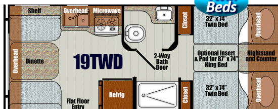
L: 23'1" Wgt: 3,035 lbs.
