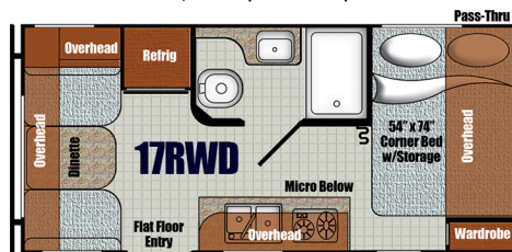
L: 20'0" Wgt: 2,567 lbs.
